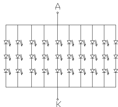
BL CIRCUIT DIAGRAM
