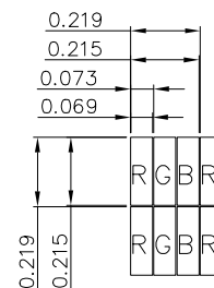
DOTS DETAIL
